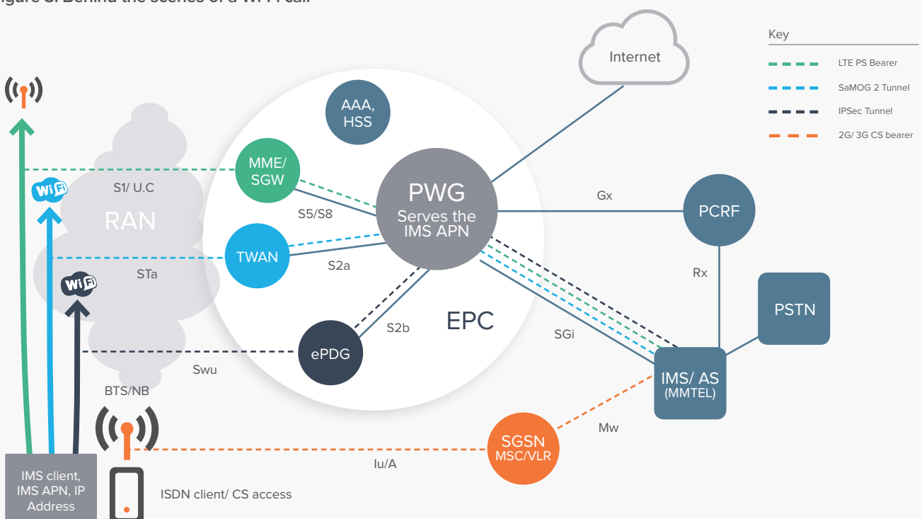
Figure 3: Behind the scenes of a Wi-Fi call
